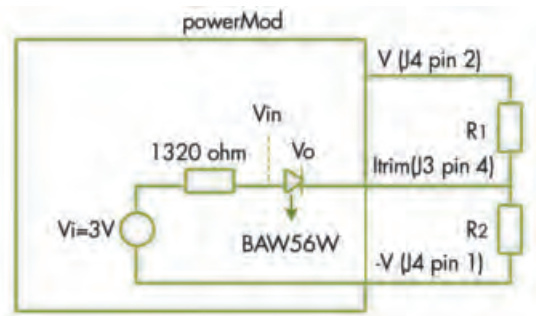
Foldback Current Limit
