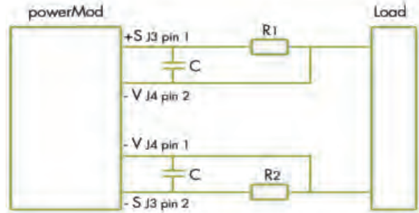
Remote Sense of Output Voltage
