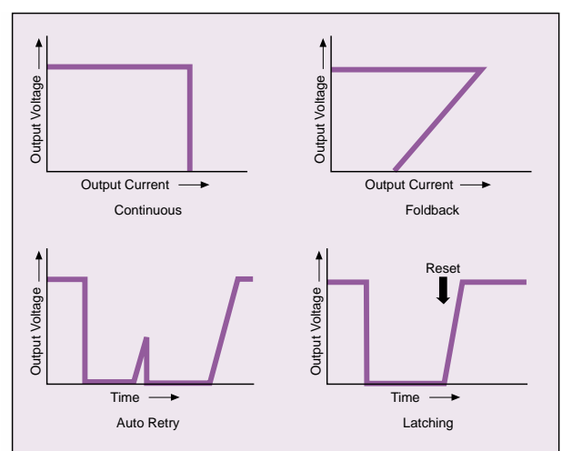
Figure 2.11 - Types of Electronic Current Limiting
