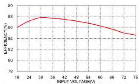
UFEC15-48S05W Efficiency vs. Input Voltage
