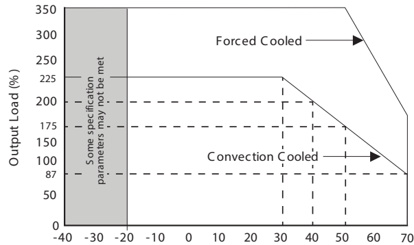
Figure 9 - GCS350
